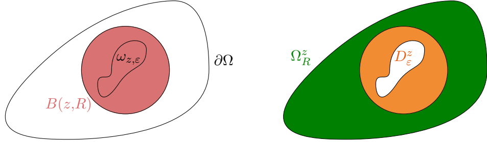
Figure 2: The truncated domain
