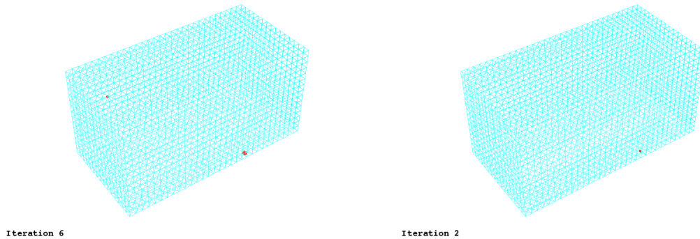
Figure 11: Detection of \omega_1^* , \omega_2^* and \omega_3^* for different measurement domains
