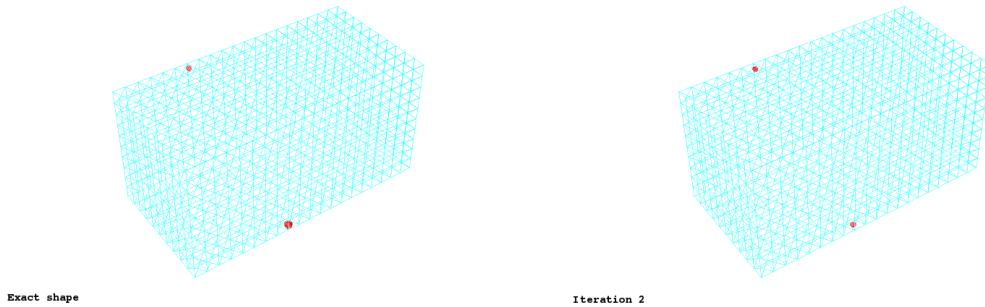
Figure 6: Detection of \omega_7^* and \omega_8^*
