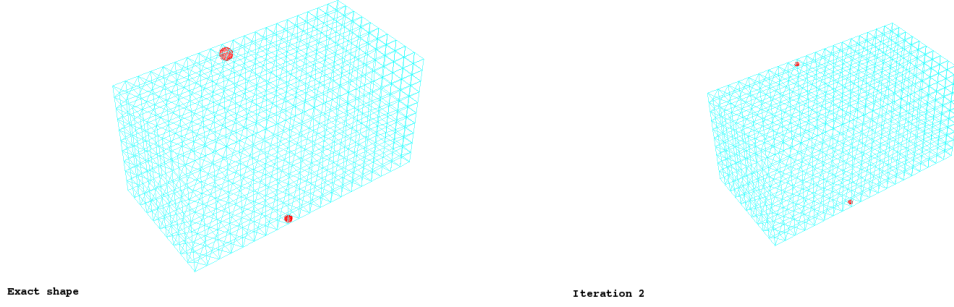
Figure 10: Detection of \omega_9^* and \omega_{10}^*
