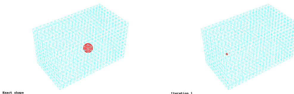
Figure 9: Detection of a big obstacle
