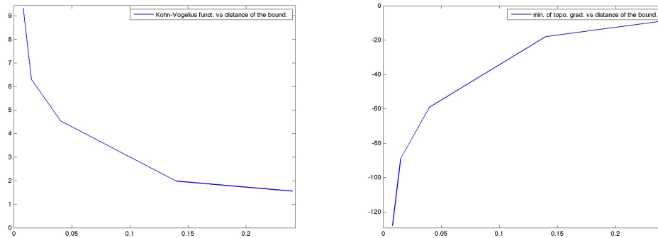
Figure 8: The initial Kohn-Vogelius functional and minimum of the topological gradient versus the distance of the obstacle from the exterior boundary d
