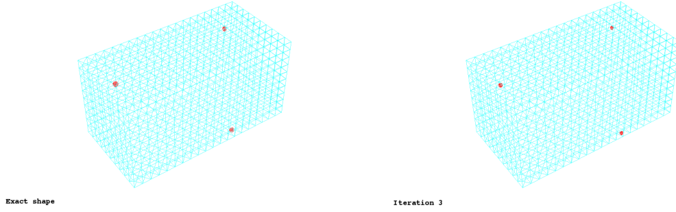
Figure 3: Detection of \omega_1^* , \omega_2^* and \omega_3^*
