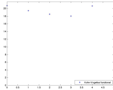
Figure 4: Evolution of the functional \mathcal{J}_{KV} during the detection of \omega_1^* , \omega_2^* and \omega_3^*
