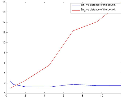
Figure 7: The Euclidean norm of the error between the exact and the approximate coordinates versus the non-dimensional distance \eta
