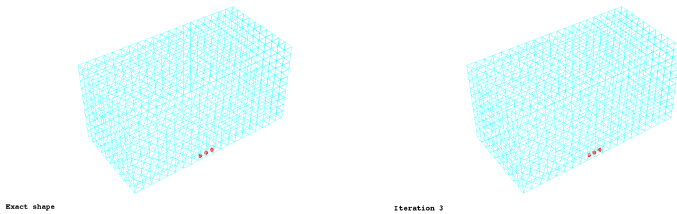
Figure 5: Detection of \omega_4^* , \omega_5^* and \omega_6^*
